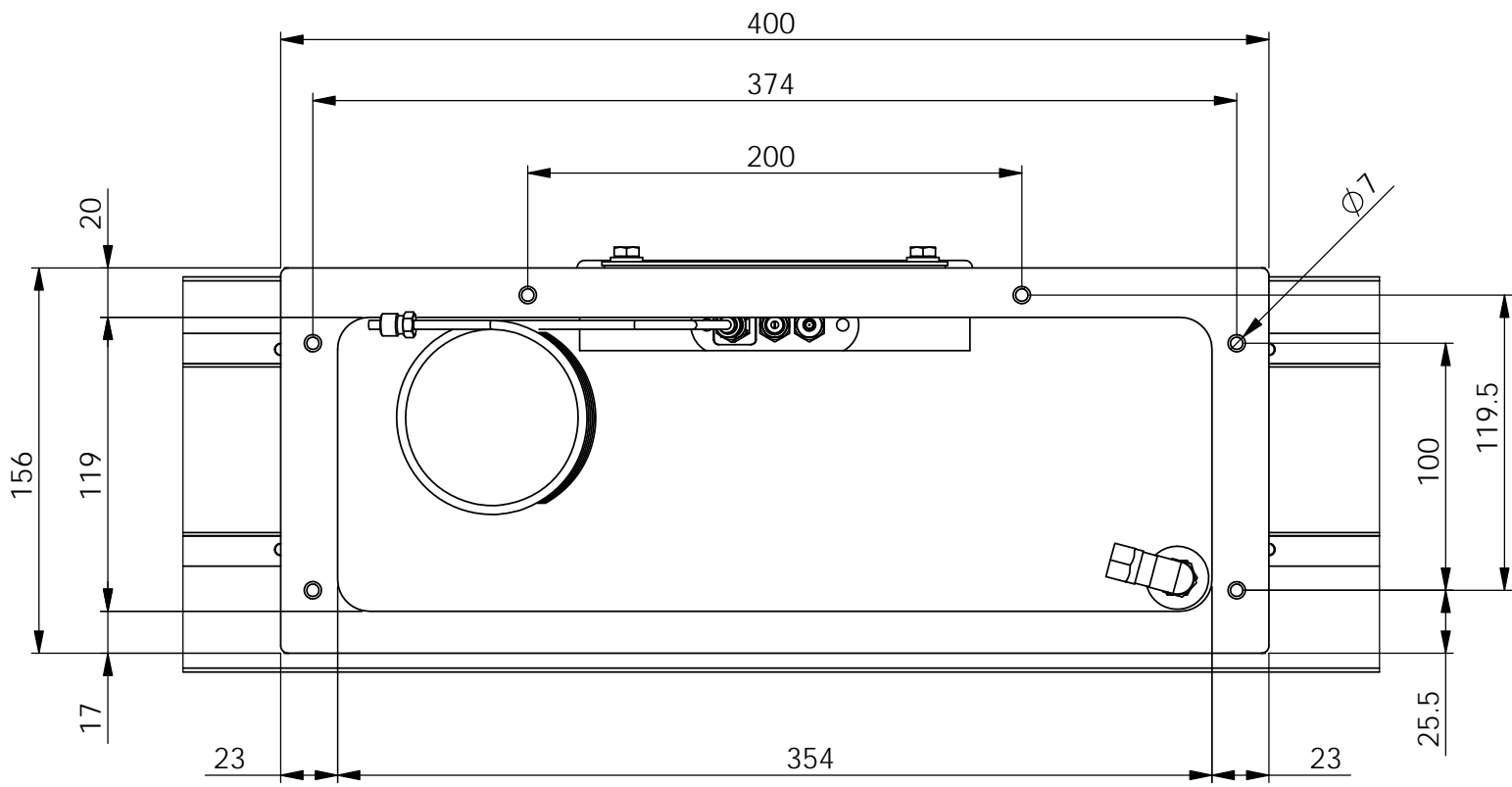
DETAIL A
