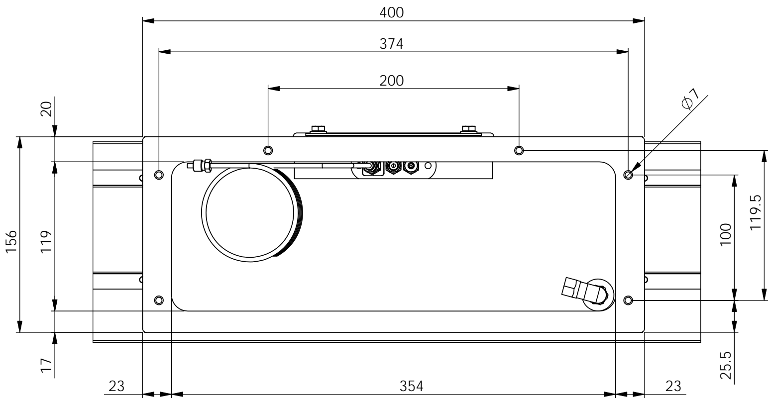
DETAIL A
